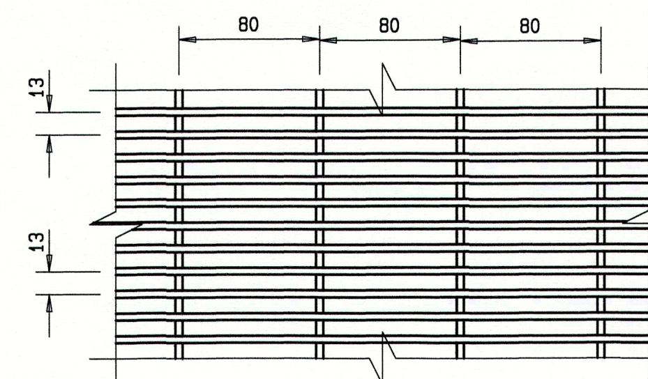
DETAIL 'A' MAXIMUM APERTURE SIZE SCALE 1:3
