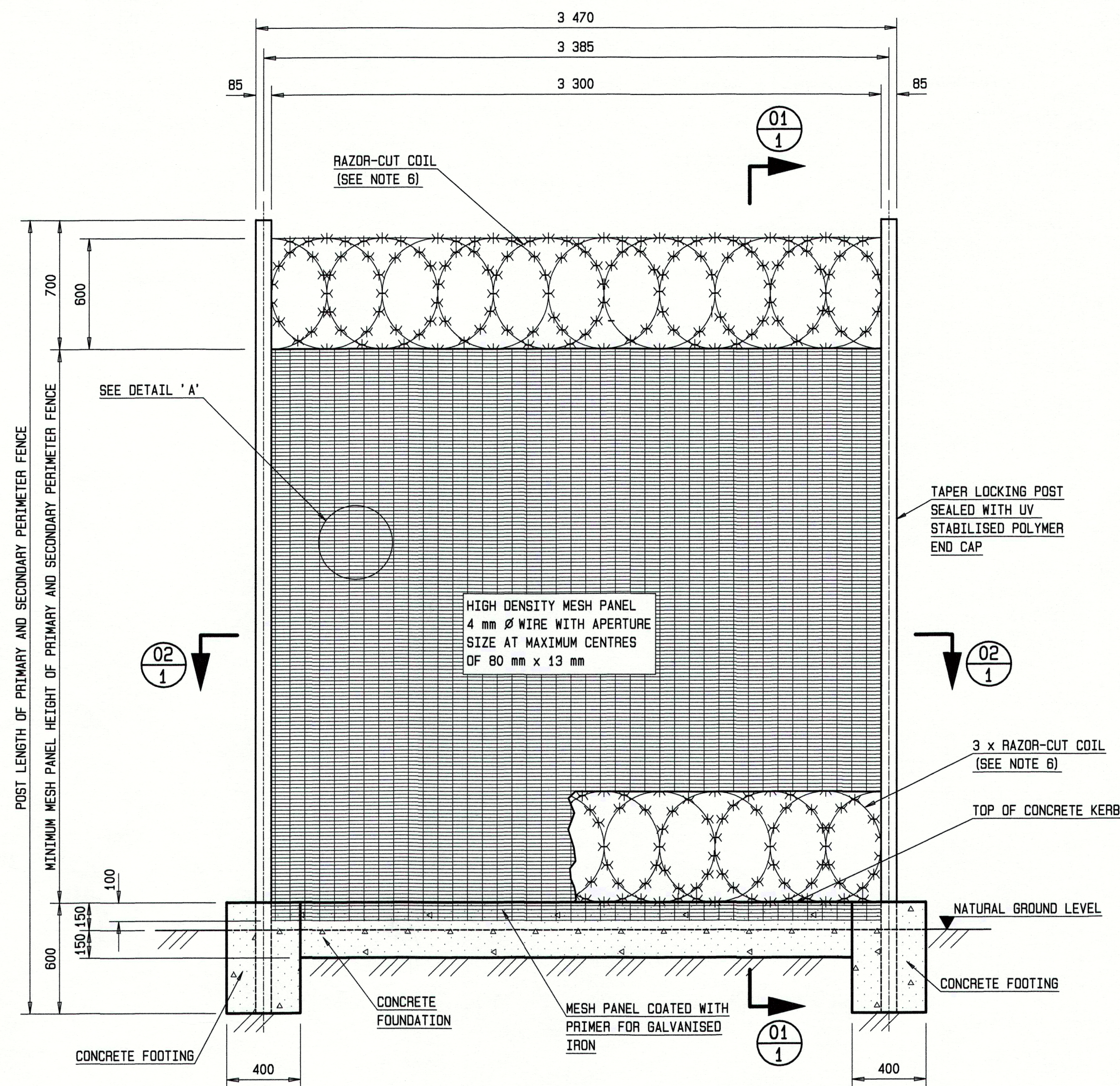
ANTI-INTRUDER FENCING SYSTEM TYPICAL ELEVATION
