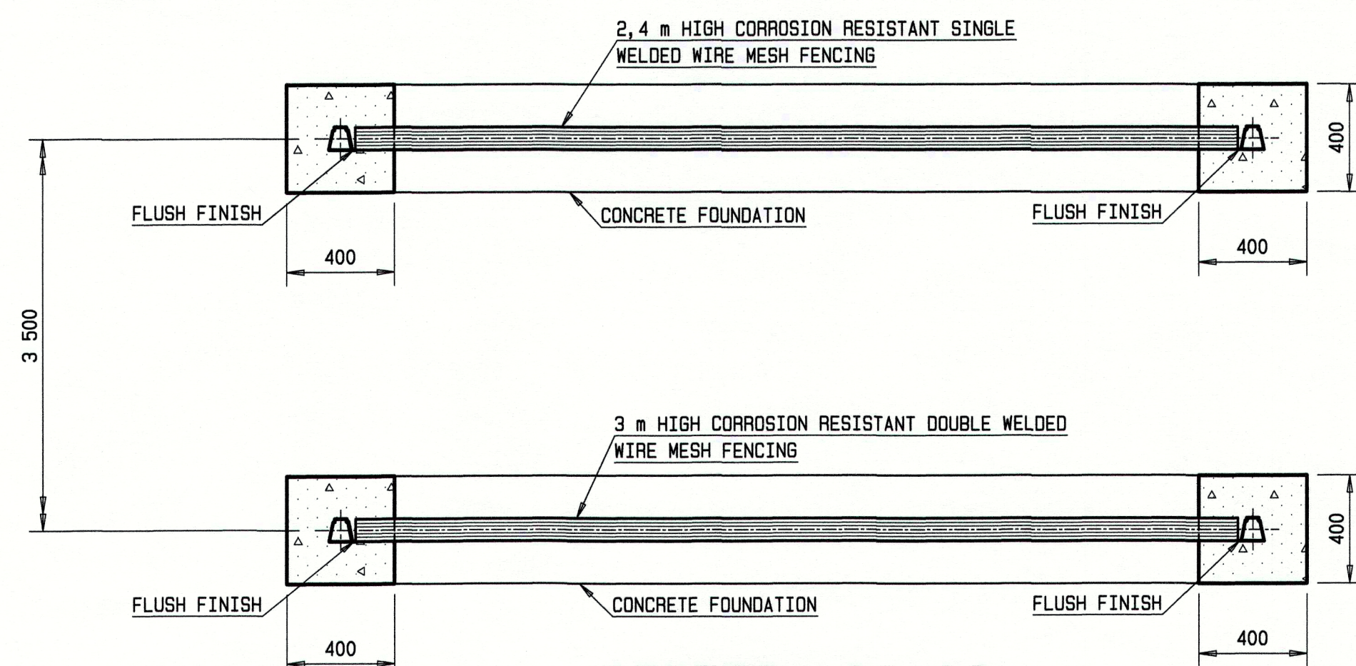
SECTION 02-02
