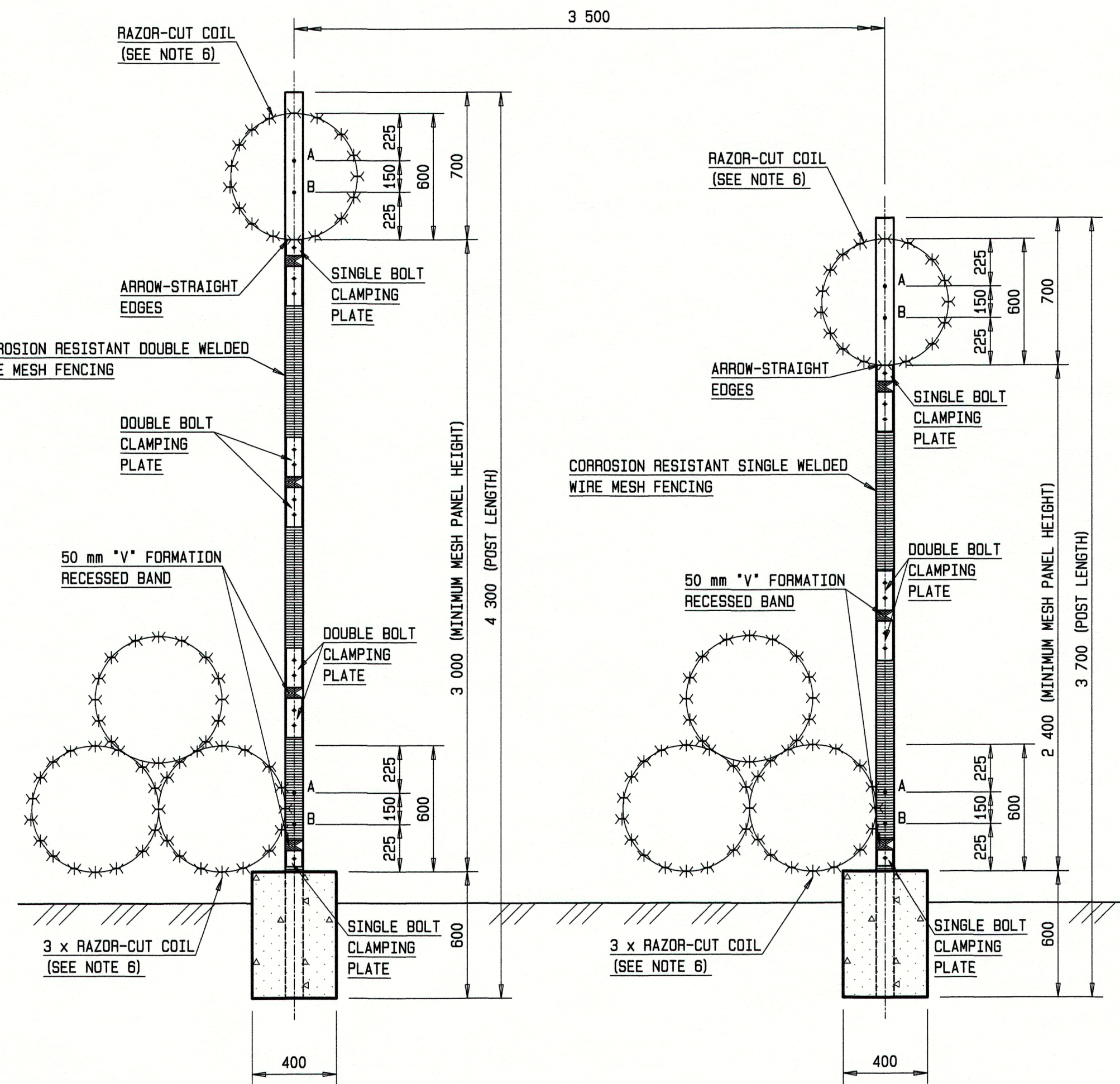
SECONDARY PERIMETER FENCING
